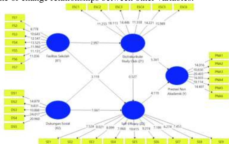
Figure 2. Evaluation of Path Analysis
