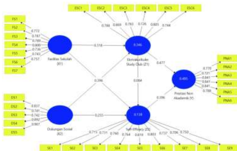
Figure 1. Evaluation of the Measurement Model
